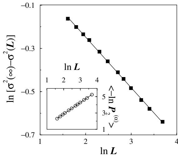
FIG. 2. \sigma^2(\infty) - \sigma^2(L) as a function of L for the Anderson transition on a log-log scale. L ranges between 5 and 40. The straight line is a linear fit to Eq. (5), and the slope is obtained from the inset. Inset: \langle \ln P_2^{(\alpha)} \rangle versus \ln L . The straight line is a linear fit to the data and its slope is equal to the (average) correlation dimension D_2 .
