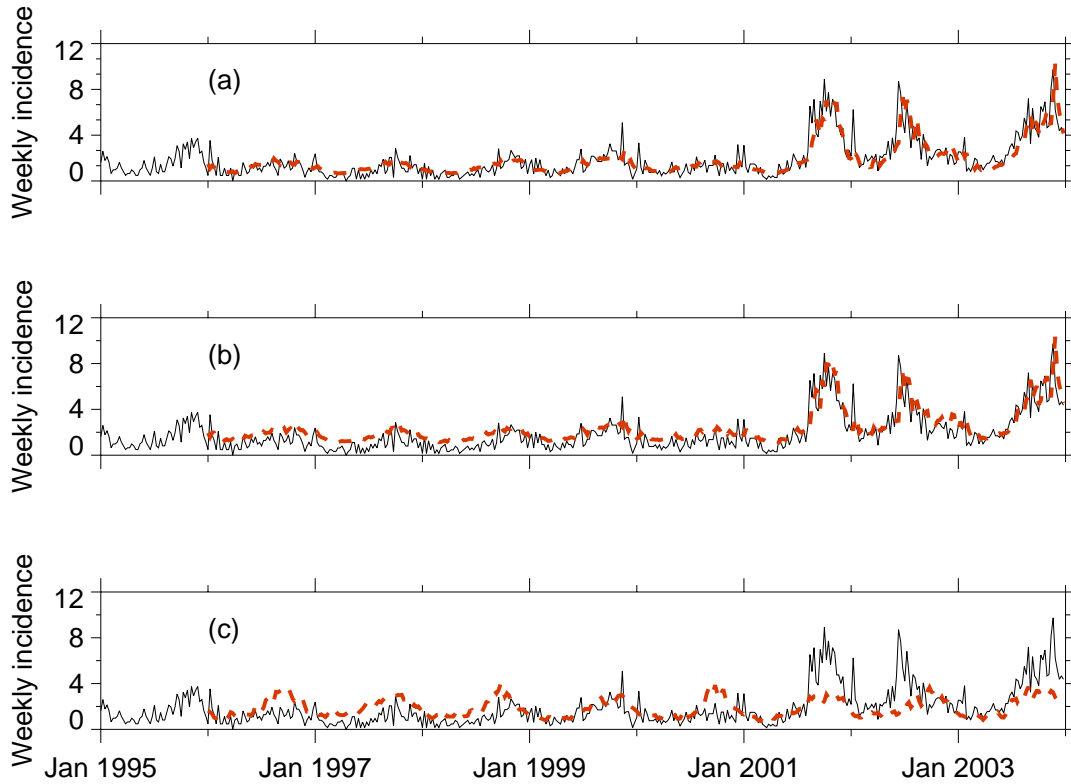
Figure 2. Reported valley fever incidence in Kern County, California (cases per 100, 000 population) and three models for the period Jan 1996- Dec 2003. In all three panels, thin solid lines indicate incidence, and dashed heavy lines correspond to model results: (a) full model, (b) final model, and (c) environmental model. The year 1995 is missing from the model results because they require at least one year of valley fever incidence data to start predicting future values.
